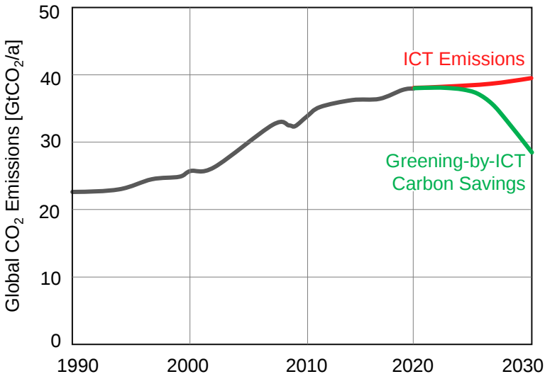
Global greenhouse gas emissions according to [ourworldindata.org/co 2 -and-other-greenhouse-gas-emissions] and the ICT emissions from the previous diagram as well as the possible emission savings according to #SMARTer2030 – ICT Solutions for 21st Century Challenges from GeSI.
